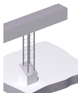
Poteaux
